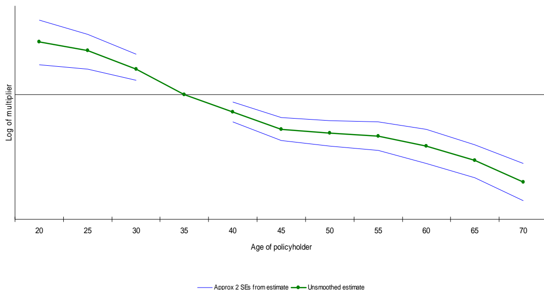
Poisson multiplicative lapse model output
