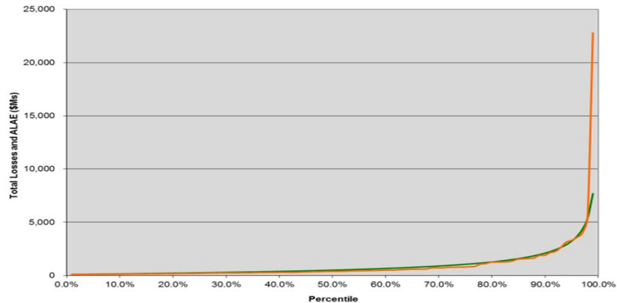
Empirical GL Claims vs Pareto Distribution
